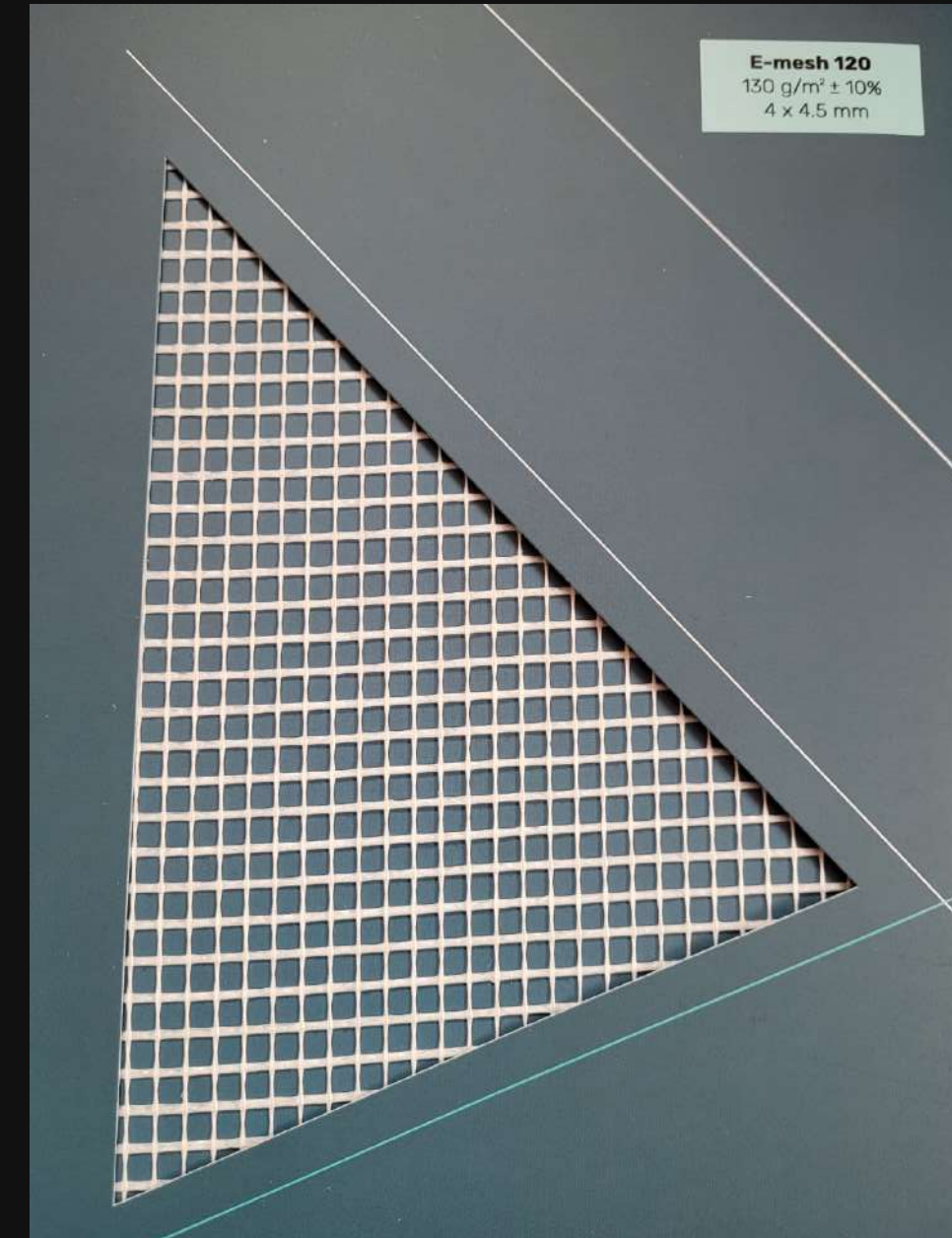
FIBERGLASS MESH 130G/M2 4MM X 4,5MM
