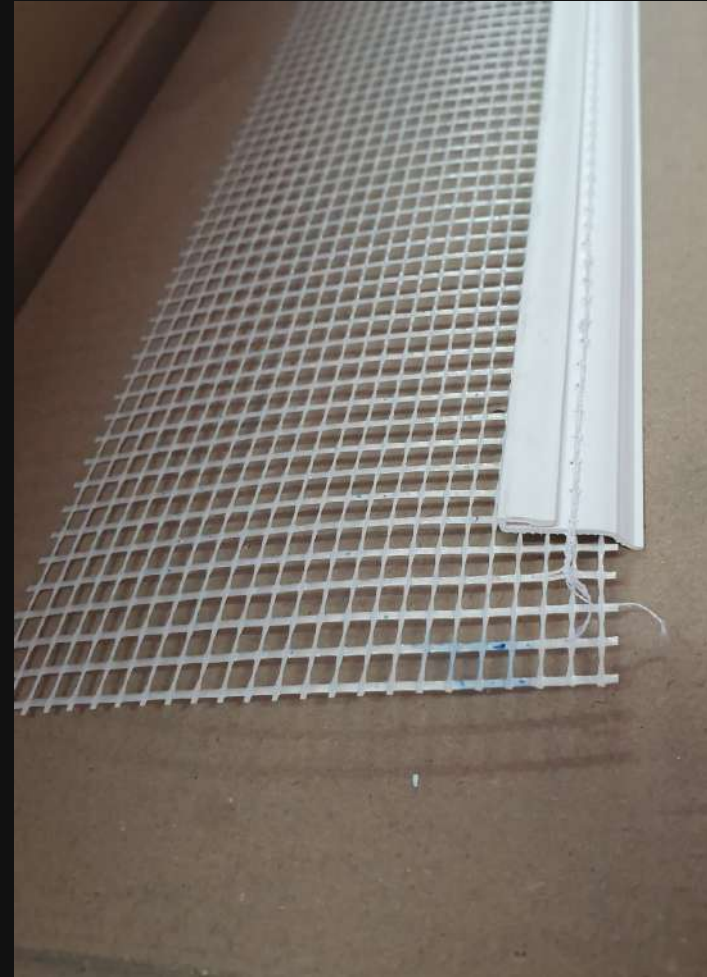
PVC DRIP NOSE PROFILE PINNED TO SOCLE PROFILES 3MM OR 6 MM
