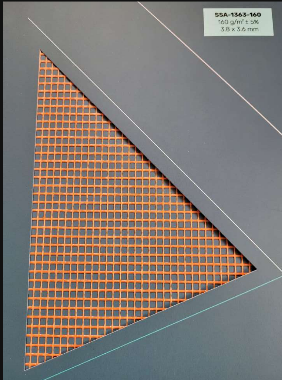
FIBERGLASS MESH 160G/M2 3,8MM X 3,6MM
