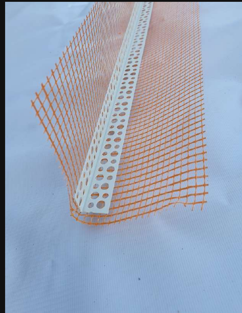
PVC CORNER WITH MESH LUX 20 CM OR 25 CM ( 145G/M2) Lenght 2,5 m
